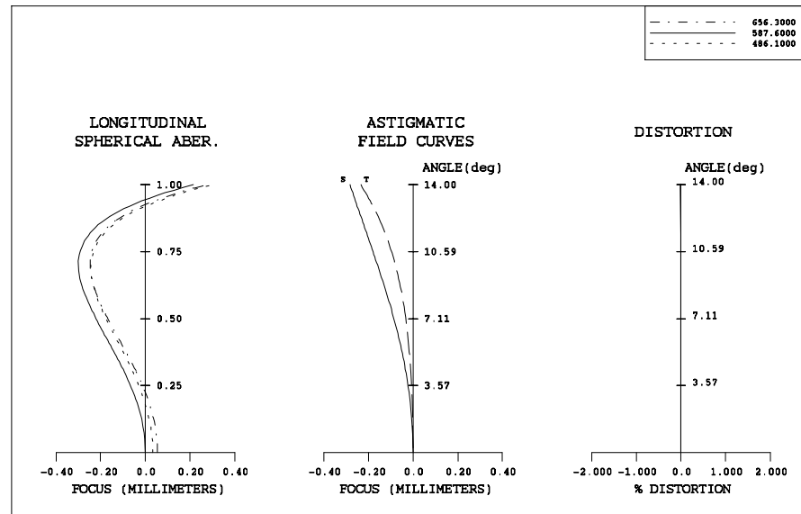
Double Gauss - U.S. Patent 2,532,751
